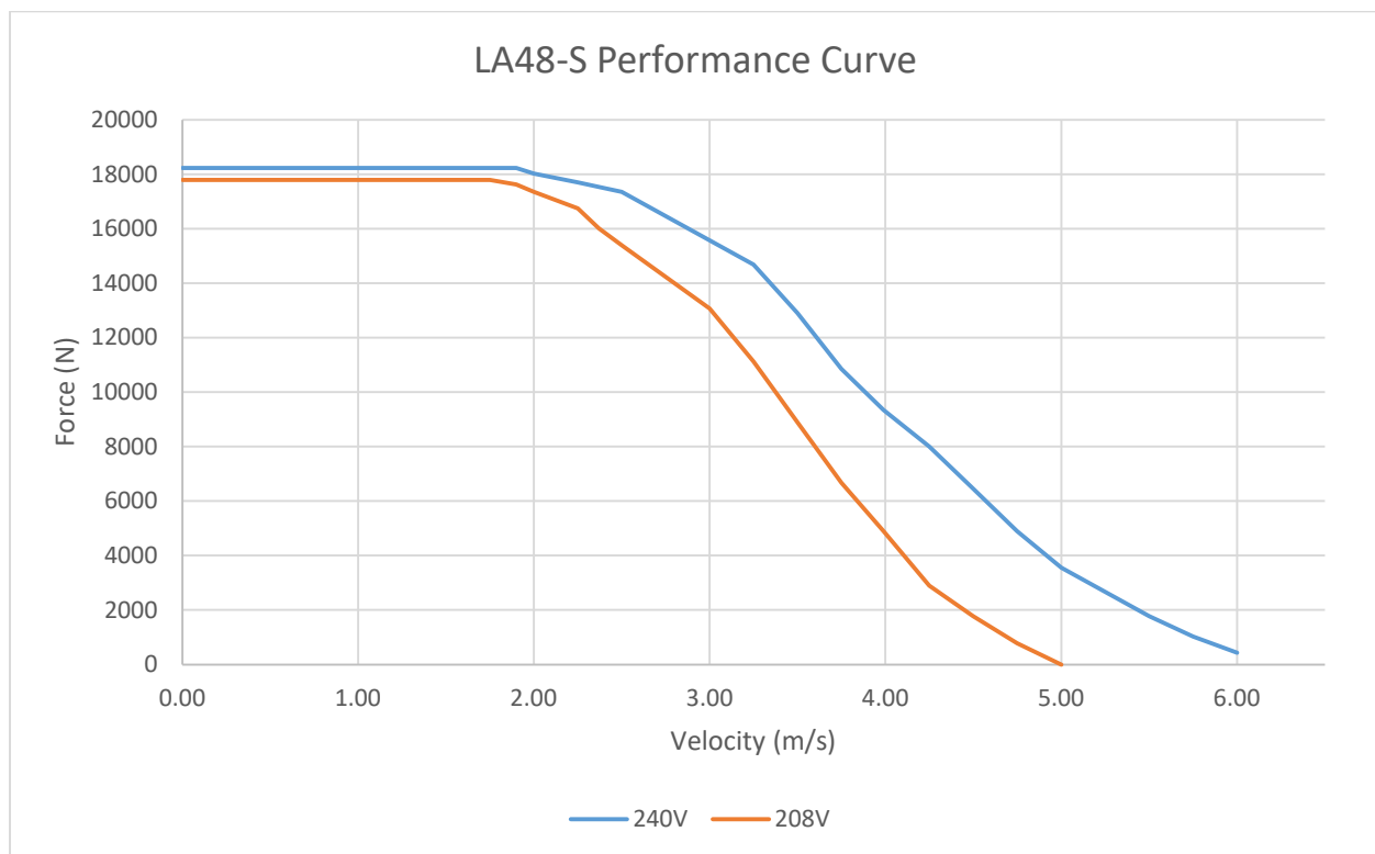
LA 48 Peak Power and Performance Curve – Metric units
